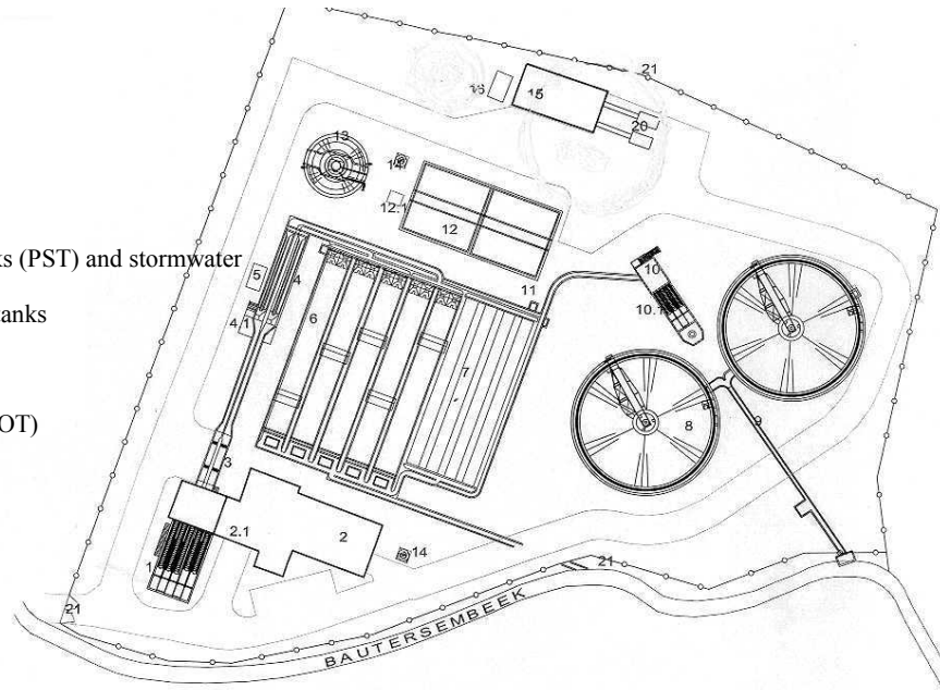
Figure 2. Layout of the WWTP Hove
