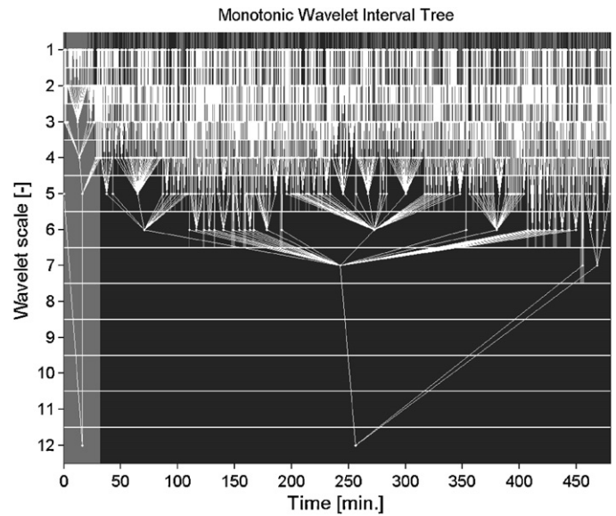
Fig. 8. Construction of the Wavelet Interval Tree (WIT, step 3) – Monotonic Wavelet Interval Tree (MWIT). White lines visualize the interval tree explicitly.
