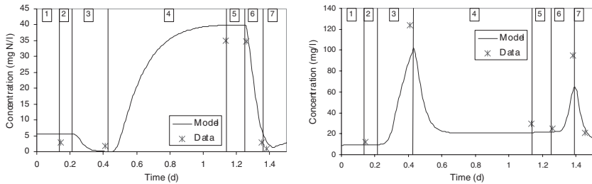
Figure 3 Measured and simulated nitrate (left) and readily biodegradable COD (right) concentration during the nitrate addition test ( D_{f,SS} = 0.28 \text{ cm}^2/\text{d} ) (numbers indicate phases given in Table 1)
