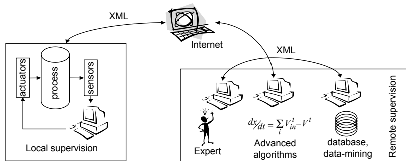
Figure 1 The overall architecture of the TELEMATC supervision system
