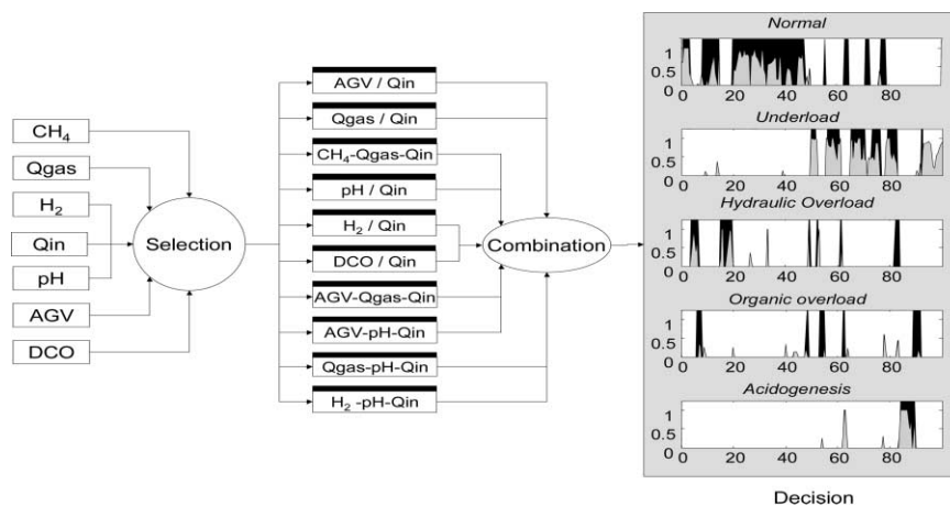
Figure 5 Illustration of the results provided by the TELEMAT fault detection and diagnosis system
