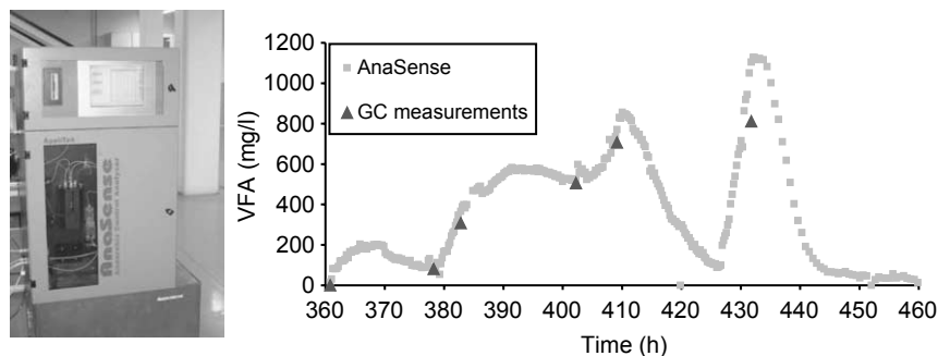
Figure 2 Validation of the AnaSense sensor dedicated to the measurement of VFA, bicarbonate, total and partial alkalinity
