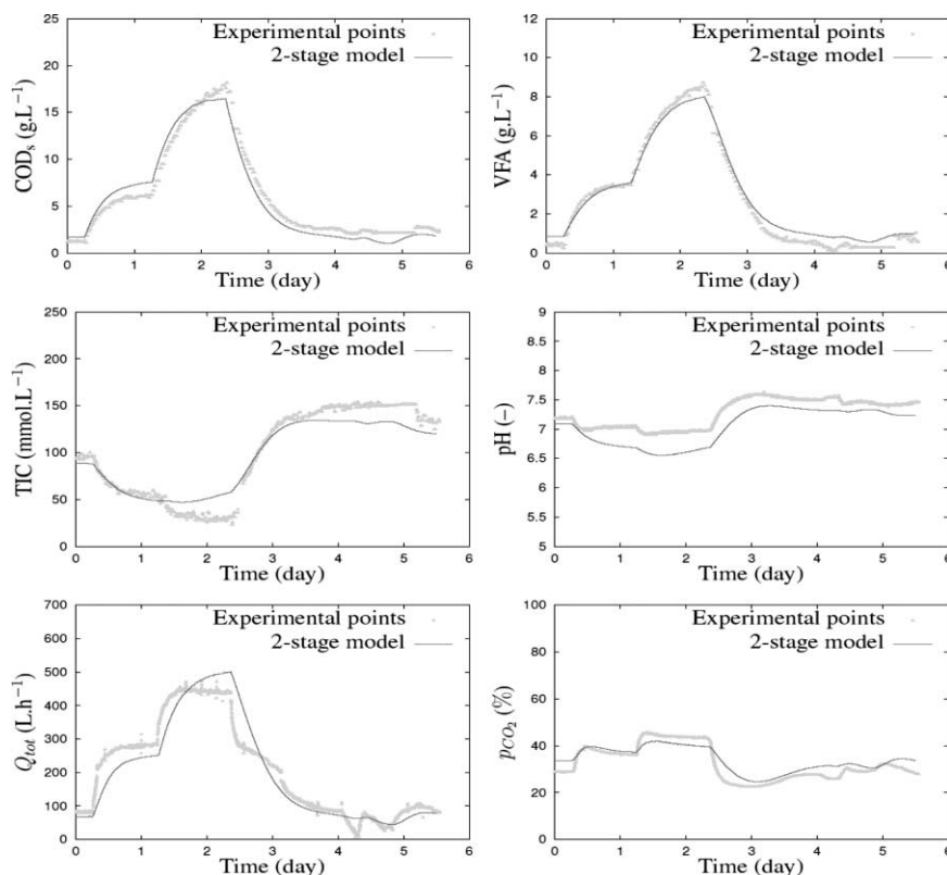
Figure 4 Experimental process overloading on a fixed bed digester processing wine vinasses. Comparison between sensor measurements and model predictions
