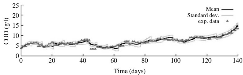
Figure 3 Software sensor validation: off-line soluble COD measurements ( \Delta ) are compared to the predictions of the software sensors (average predicted value and confidence interval)
