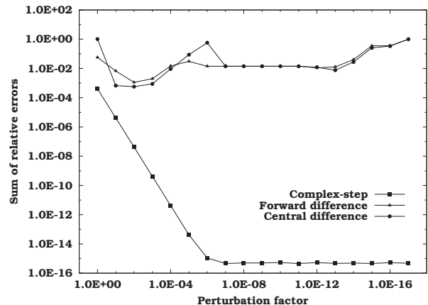
Fig. 3. Sum of relative errors of the sensitivity function \partial S_2 / \partial K_{S_2} of the anaerobic digestion model for the complex-step derivative approximation method, forward difference and central difference.
