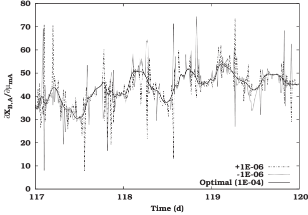
Fig. 2. Numerical error effect: sensitivity of the Benchmark autotrophic biomass ( X_{B,A} ) to the maximum autotrophic growth rate ( \mu_{m,A} ) calculated with perturbation factors \pm 1E-06 and 1E-04 .
