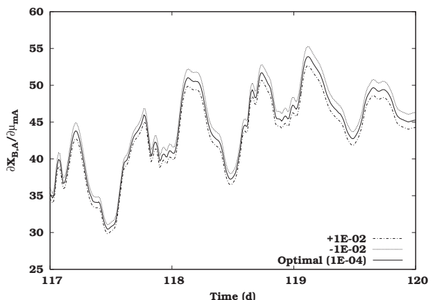
Fig. 1. Nonlinear effect: sensitivity of the Benchmark autotrophic biomass ( X_{B,A} ) to the maximum autotrophic growth rate ( \mu_{mA} ) calculated with perturbation factors \pm 1E-02 and 1E-04 .
