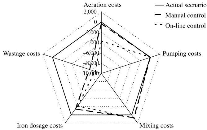
Figure 4 Effect of manual and on-line control expressed as absolute values
