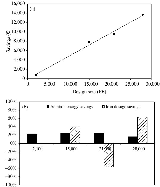
Figure 6 Cost reductions in function of plant size: total savings (a), relative savings (b)
