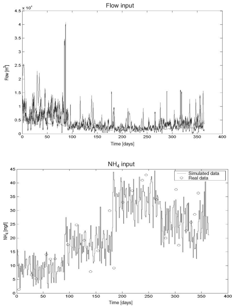
Figure 2 Example of a synthetically generated influent series versus real data
