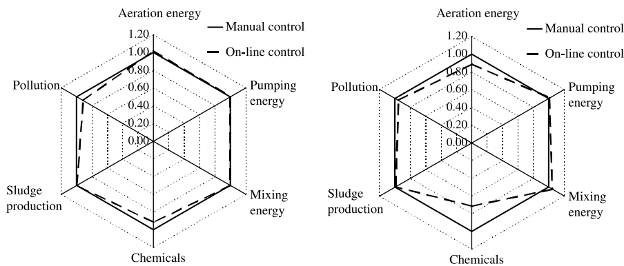
Figure 5 Effect of overload (left) and underload (right) situations. Manual control is taken as a reference.
