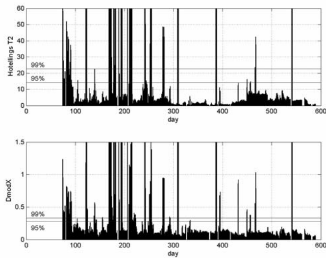
Figure 2: Hotelling's T^2 and DmodX (distance to the model plane) control charts based on the selected model 1
